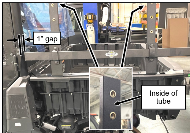
Fig. 9; Install Tool Rack's Vertical Tubes.
