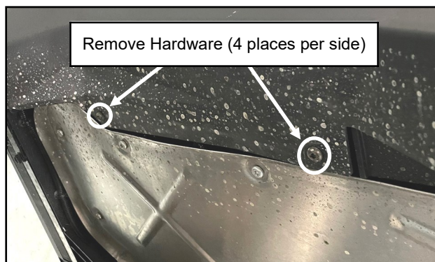
Fig. 5; Remove Underside Screws on the Side Panel
