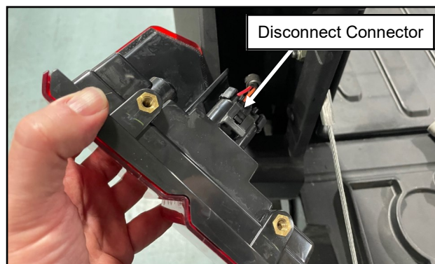
Fig. 3; Disconnect Left Tail Light
