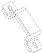
TUBE CLAMP ASS'Y. P/N: 8SV-110-00068 (QTY.: ONE)
