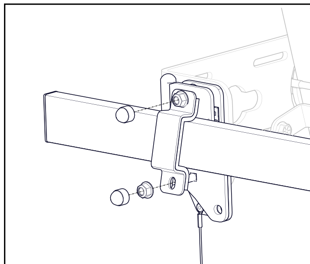
Fig. 6 (Attach Bar to Brackets)
