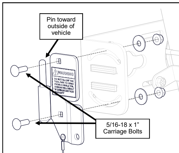
Fig. 3 (Attach Pin Brackets to ROPS Brackets)
