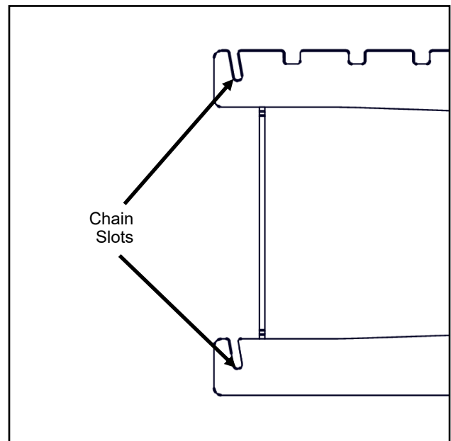
Fig. 8; Chain Slots on Fork Frame (Right Side)
