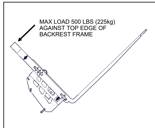
Fig. 4; Max Load on Backrest Frame
