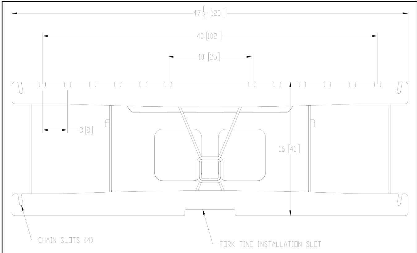
Pallet Fork Frame, Mini Skid Steer Dimensions (inches [cm])
