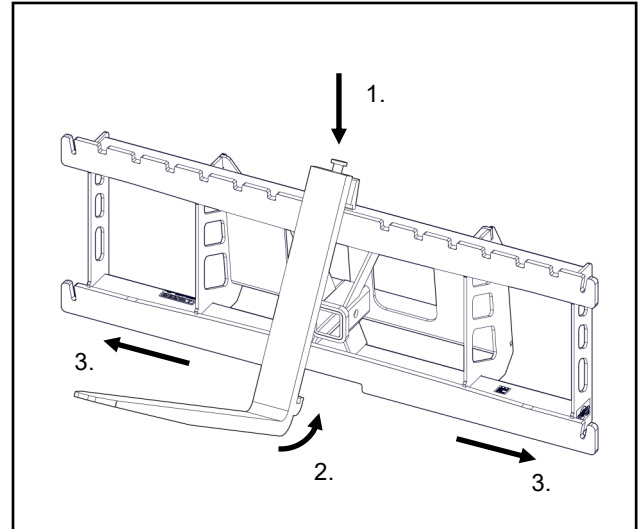
Fig. 2; Install Fork Tines
