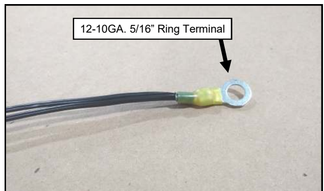
Fig. 18 (5/16" Ring Terminal to Black Wires)
