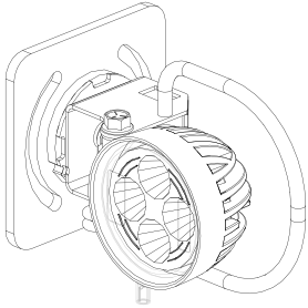
ROPS MOUNTED LIGHT ASSY, LEFT P/N: 8SV-113-00182-L
