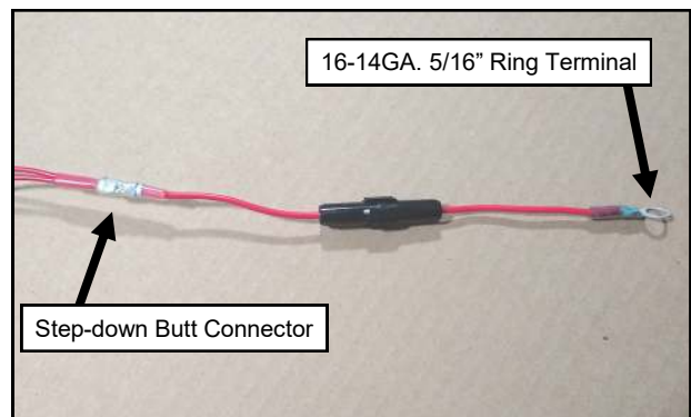
Fig. 16 (Fuse Holder Installation)
