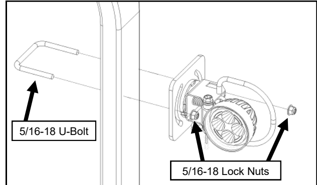
Fig. 1 (Left Light Bracket Assy. Orientation)
